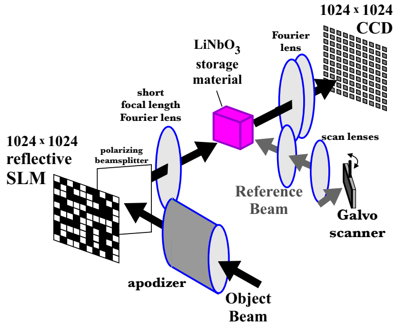
Figure 3: Salient features of the DEMON II holographic digital data storage engine. Utilizing 30mm focal length Fourier transform lenses in the 90 degree geometry with a 1 million pixel SLM, this system has demonstrated an areal storage density of nearly 400 bits per square micron.
