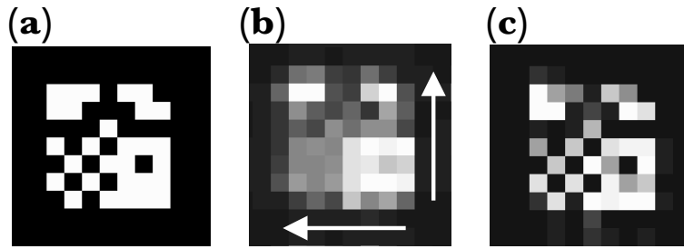
Figure 6: A 9 \times 9 pixel pattern is imaged from SLM to CCD (a) under perfect conditions; (b) with half-a-pixel offset in both x and y ; (c) after post-processing with the shift-compensation algorithm [22].
