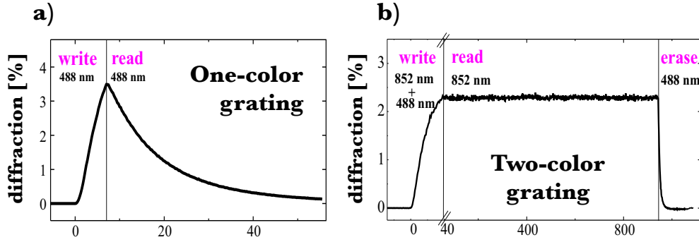
Figure 10: Typical write-read-erase curve for holographic gratings in LiNbO 3 crystals. (a) One-color scheme, in which an argon ion laser at 488nm, 1W/cm 2 is used for both writing (two beams) and reading (one beam). (b) Two-color scheme, in which a laser diode at 852nm (4W/cm 2 total intensity) is used for writing and an argon ion laser at 488nm, 1W/cm 2 is used for the gating step. Nondestructive reading was done with one of the unattenuated writing beams (2W/cm 2 ) and erasing with the gating light [41].
