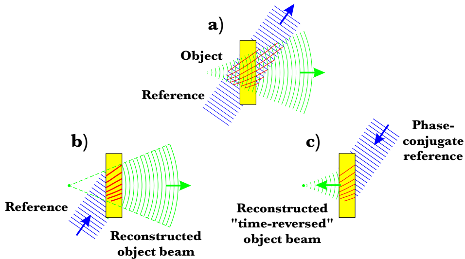
Figure 1: How to record and read data using holograms: (a) Holographic storage of a single data bit. The spherical wave from a single pixel interferes with a coherent plane wave in the reference beam. The resulting interference pattern changes the refractive properties of the photosensitive medium. (b) The hologram is read out using the original reference beam, which is diffracted by the stored interference pattern to reconstruct the original spherical wavefront. An image of this beam can be formed on a single detector pixel, resulting in the retrieval of a single bit. (c) The hologram can also be read out by illuminating it with a counter-propagating (or “phase-conjugate”) reference beam, which reconstructs a phase-conjugate copy of the original object beam. This beam returns to its original point of origin, where the bit value can be read without requiring a high-quality imaging system.
