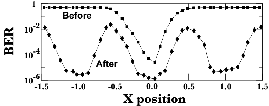
Figure 7: Dependence of raw-BER (with an 8:12 modulation code [12]) before and after shift-compensation post-processing, as a function of x shift [22].
