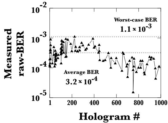
Figure 5: Measured raw-BER results from the DEMON II tester at high areal density [20].
